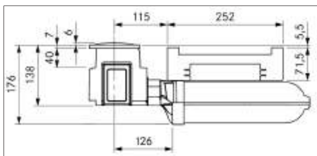
Fig. 3.2 PKA3/PKA3AB appliance dimensions front view
