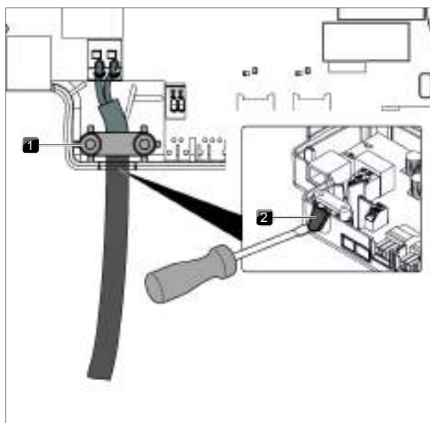
Fig. 4.65 Home Out contacts with strain relief
