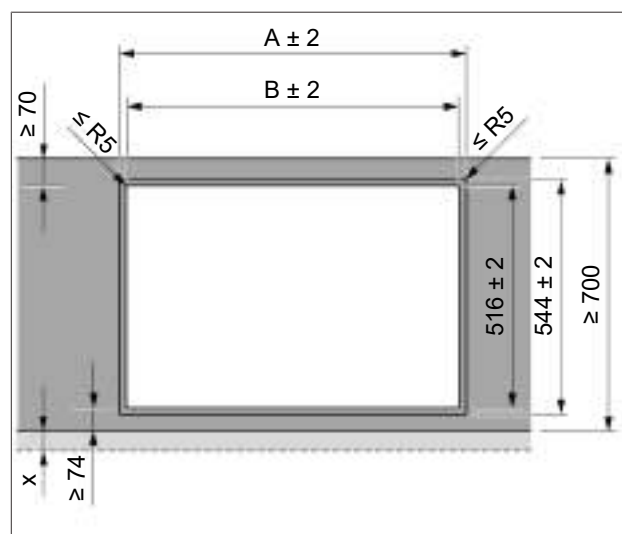
Fig. 4.11 Cut-out dimensions for flush installation
