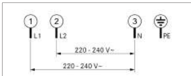
Fig. 4.88 2-phase connection diagram
