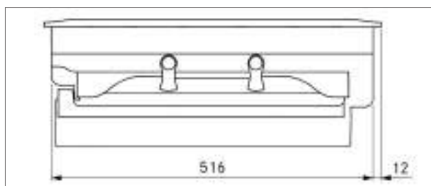
Fig. 3.7 PKAS3/PKAS3AB appliance dimensions side view
