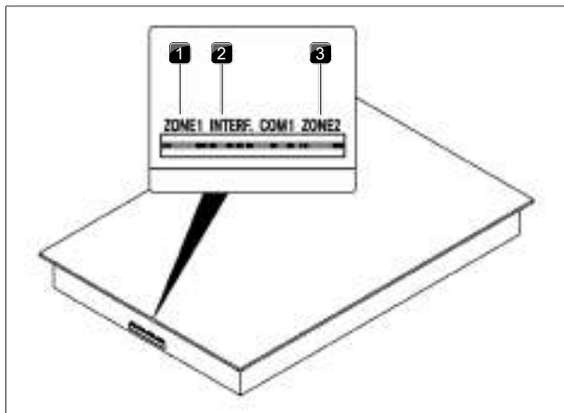
Fig. 4.71 Ports on the cooktop
