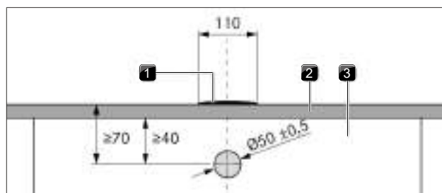
Fig. 4.16 Cooktop extractor drilling pattern
