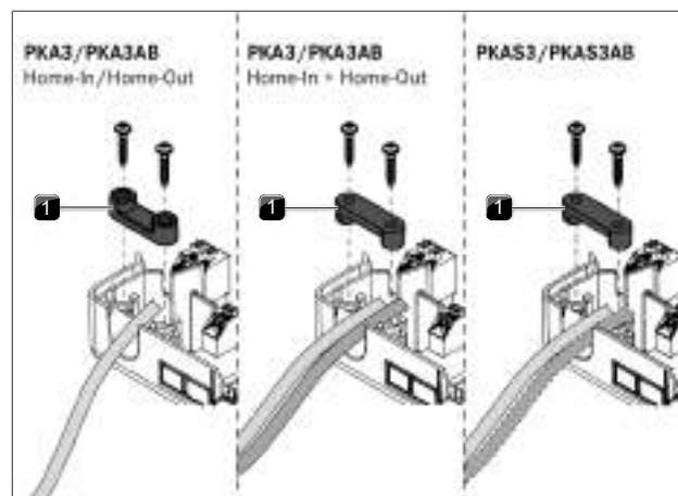
Fig. 4.68 Fitting the strain relief clamp
