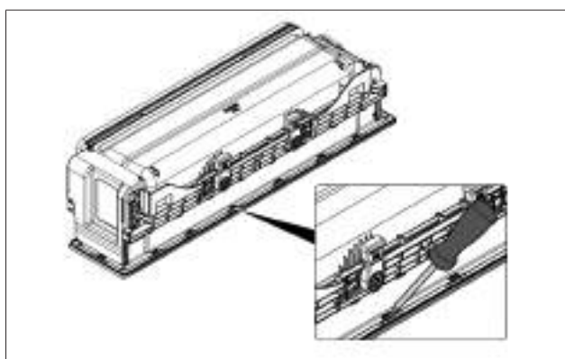
Fig. 4.29 Removing the cover frame
