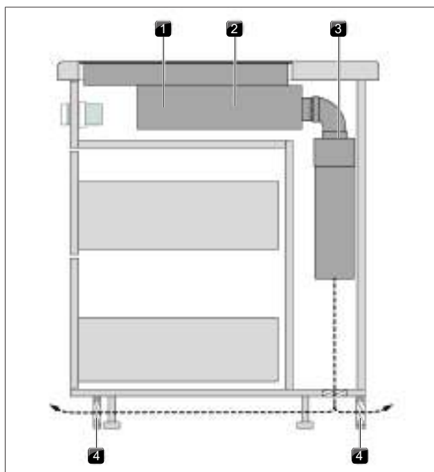
Fig. 4.9 Example of recirculated-air-return-flow planning
