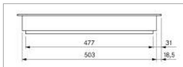
Fig. 3.28 PKT3 appliance dimensions side view
