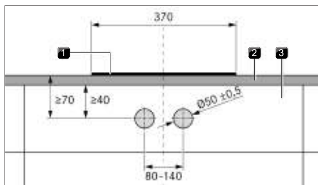
Fig. 4.17 Cooktop drilling pattern
