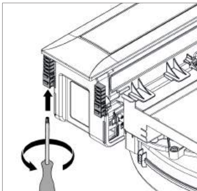
Fig. 4.37 Tightening the mounting clamps
