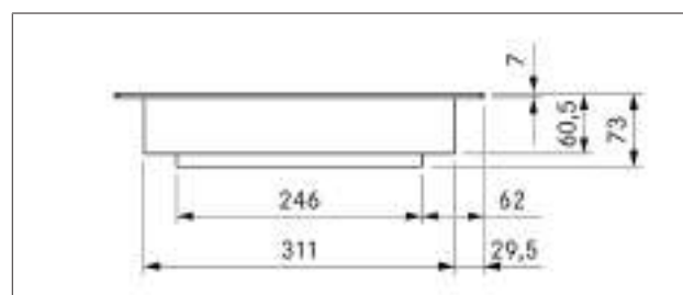
Fig. 3.27 PKT3 appliance dimensions front view
