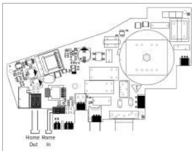
Fig. 4.64 Connection diagram for the external switch contacts
