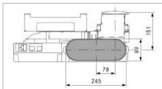
Fig. 4.41 Duct connection dimensions for PKAS3, PKAS3AB
