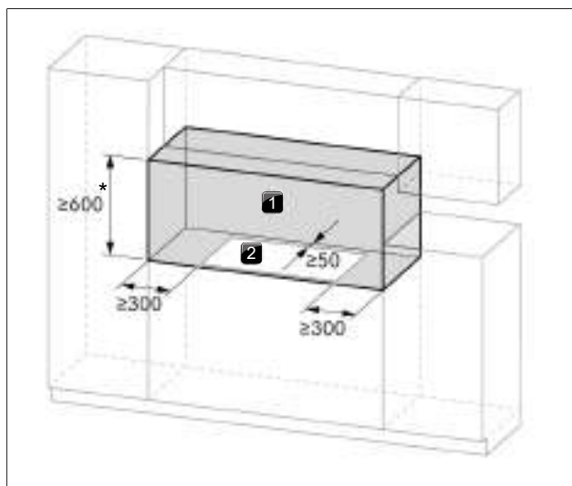
Fig. 4.3 Required clearance
