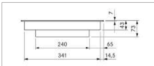
Fig. 3.21 PKCB3 appliance dimensions front view
