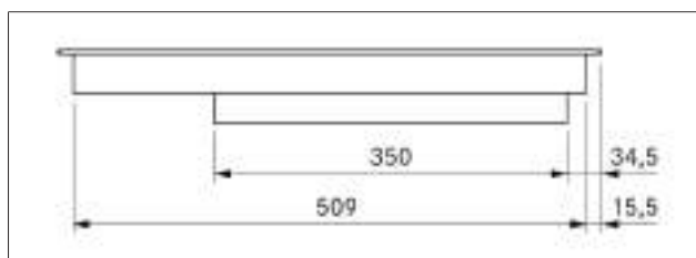
Fig. 3.22 PKCB3 appliance dimensions side view
