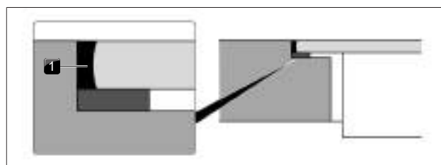
Fig. 4.89 Silicone sealant for flush installation
