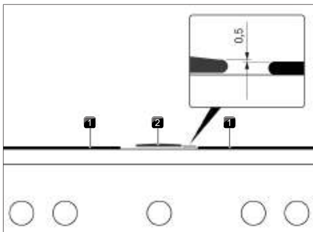
Fig. 4.33 Height difference
