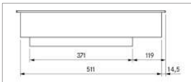
Fig. 3.16 PKIW3 appliance dimensions side view
