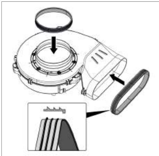
Fig. 4.43 Fitting the seals on the plinth fan
