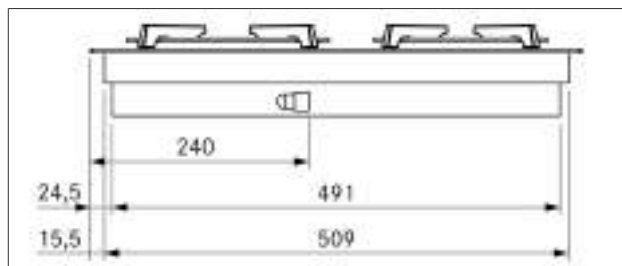
Fig. 3.31 PKG3 appliance dimensions side view
