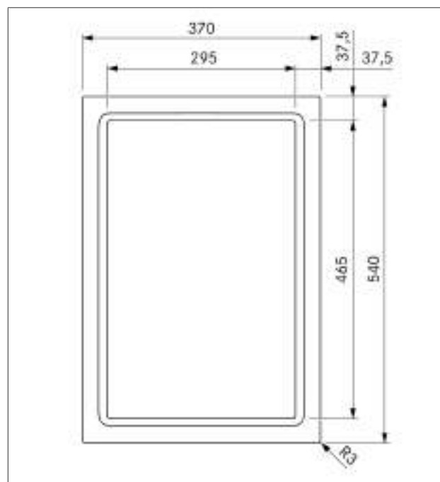
Fig. 3.26 PKT3 appliance dimensions from above
