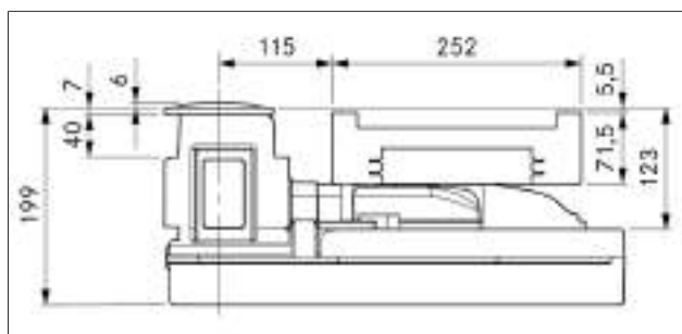
Fig. 3.6 PKAS3/PKAS3AB appliance dimensions front view
