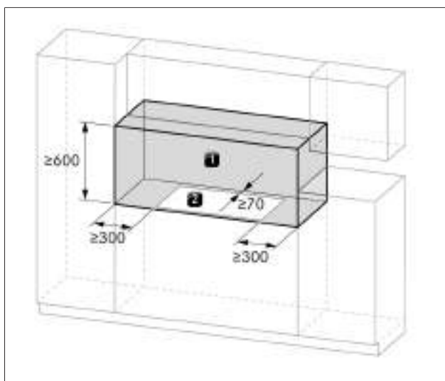
Fig. 4.57 Required clearance
