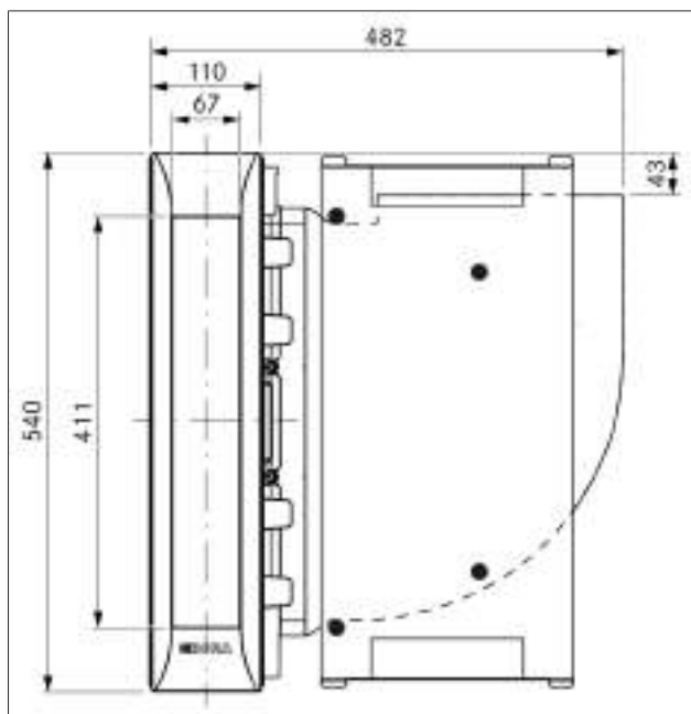
Fig. 3.1 PKA3/PKA3AB appliance dimensions from above
