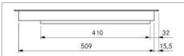
Fig. 3.10 PKI3 appliance dimensions side view
