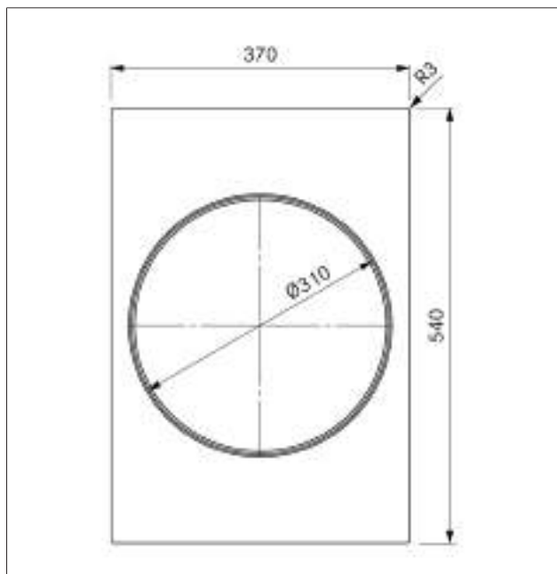
Fig. 3.14 PKIW3 appliance dimensions from above
