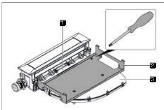
Fig. 4.24 Removing the holding plate
