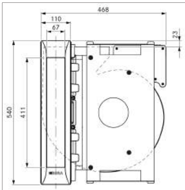
Fig. 3.5 PKAS3/PKAS3AB appliance dimensions from above
