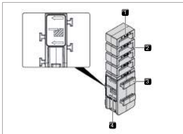
Fig. 4.34 Mounting bracket - right side (flush installation)
