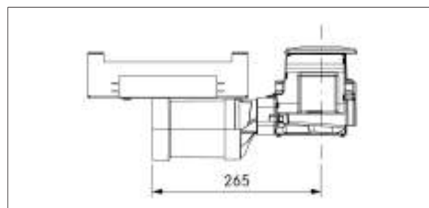
Fig. 4.40 Duct connection dimensions for PKA3/PKA3AB with the straight duct piece
