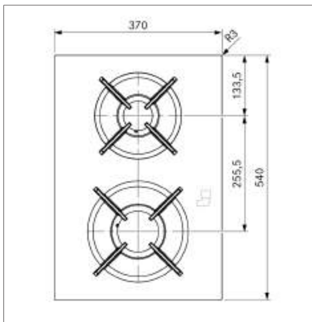
Fig. 3.29 PKG3 appliance dimensions from above
