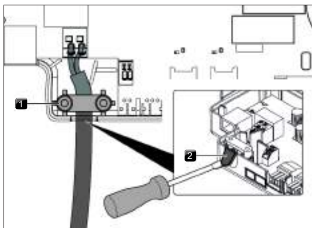
Fig. 4.67 Home Out contacts with strain relief
