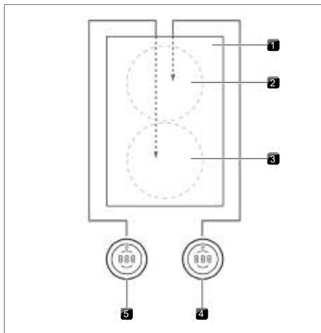
Fig. 4.73 Connecting the cooking zones when the cooktop is installed rotated by 180° and the ports are on the front of the appliance
