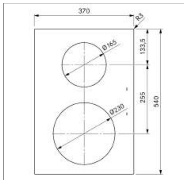
Fig. 3.11 PKI3 appliance dimensions from above
