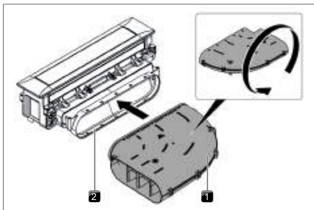
Fig. 4.27 Turning the curved duct piece over
