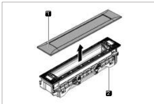
Fig. 4.30 Removing the cover frame
