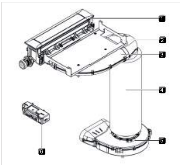
Fig. 4.44 Standard set-up for PKA3/PKA3AB
