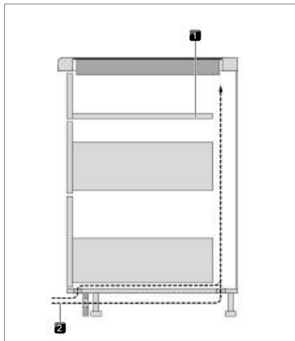
Fig. 4.8 Plinth area air supply
