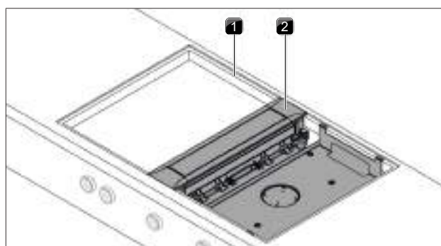
Fig. 4.31 Fitting the cooktop extractor
