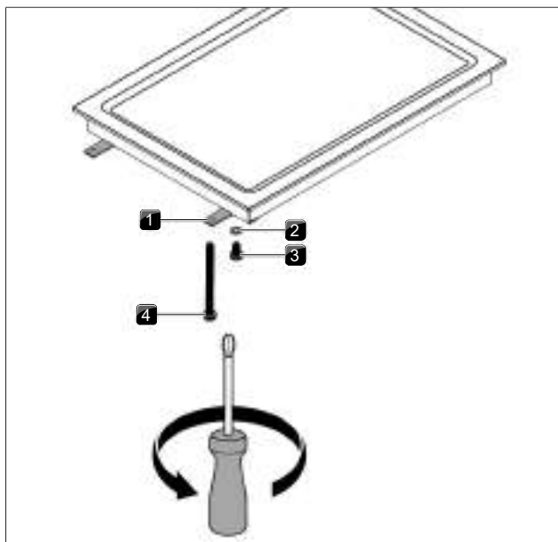
Fig. 4.56 Mounting brackets
