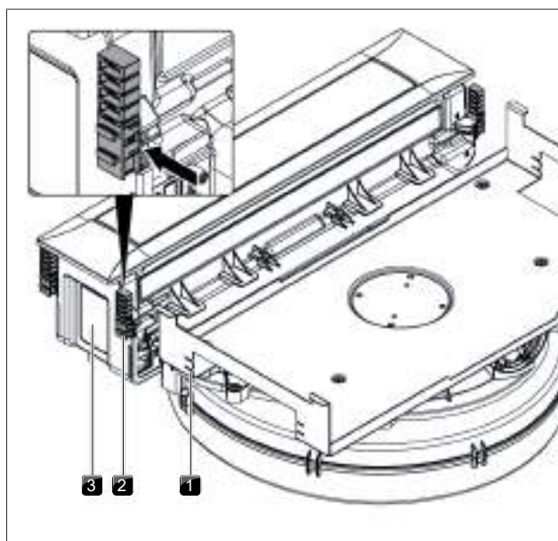
Fig. 4.36 Pushing on the mounting brackets
