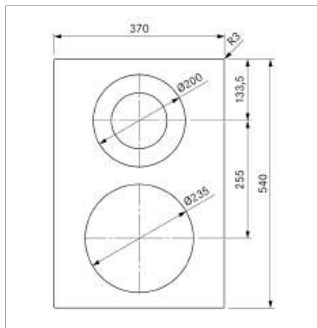
Fig. 3.23 PKCH3 appliance dimensions from above
