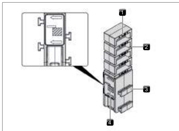
Fig. 4.35 Mounting bracket - left side (surface mounting)
