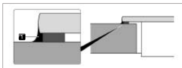
Fig. 4.90 Silicone sealant for surface mounting
