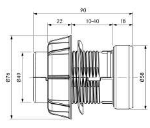
Fig. 3.33 Control knob dimensions
