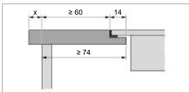
Fig. 4.10 Worktop overhang
