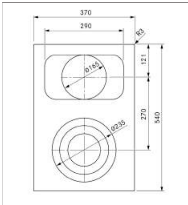
Fig. 3.20 PKCB3 appliance dimensions from above
