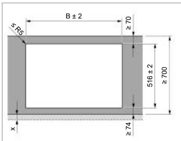
Fig. 4.13 Cut-out dimensions for surface mounting
