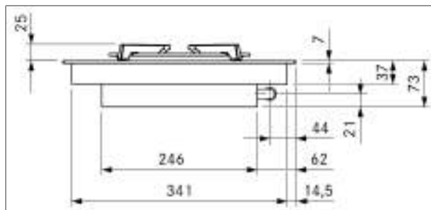
Fig. 3.30 PKG3 appliance dimensions front view
