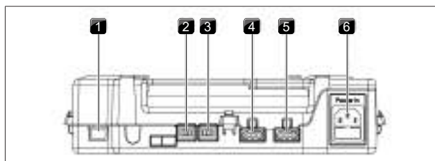
Fig. 4.81 Control unit ports
