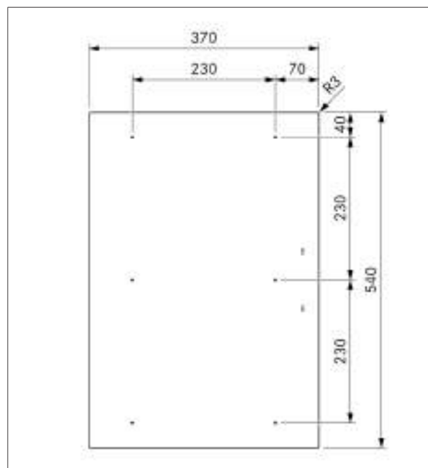
Fig. 3.8 PKFI3 appliance dimensions from above
