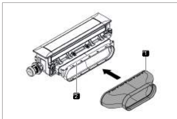
Fig. 4.26 Installing the straight duct piece
