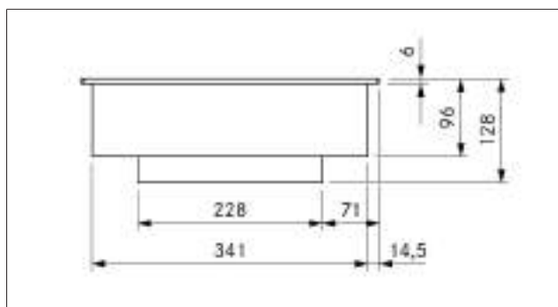
Fig. 3.15 PKIW3 appliance dimensions front view
