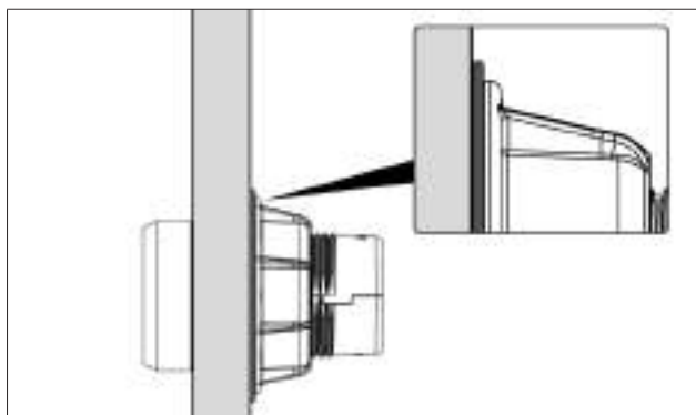
Fig. 4.23 Wave spring when installation is complete
